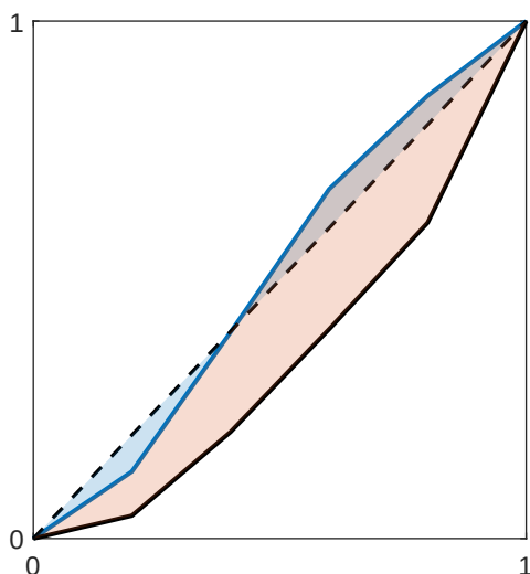
Figure 5: Geometric interpretation of the natural source decomposition of the Gini coefficient when total income consists of two sources. The solid black line depicts the Lorenz curve of total income. Shaded blue area represents the contribution to inequality due to source 1 and the shaded red area depicts the contribution of source 2. The contributions equal -0.024 and 0.318 for source 1 and 2, respectively.
