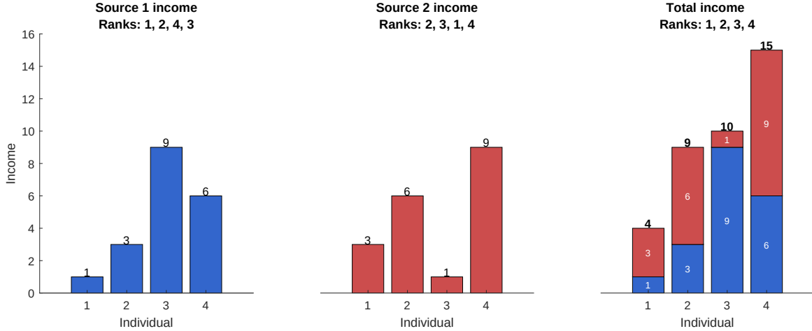
Figure 1: Income distributions of Example 1.
