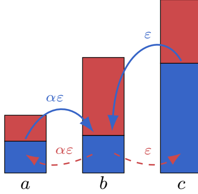
Figure 3: Illustration of compensated neutral transfers.
