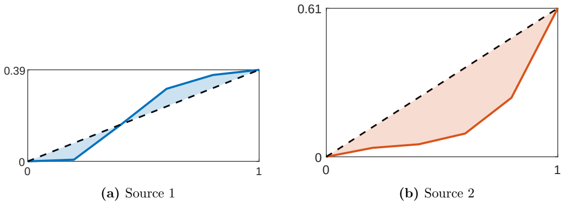
Figure 4: Normalized concentration curves of source 1 and 2 in Example 3.
