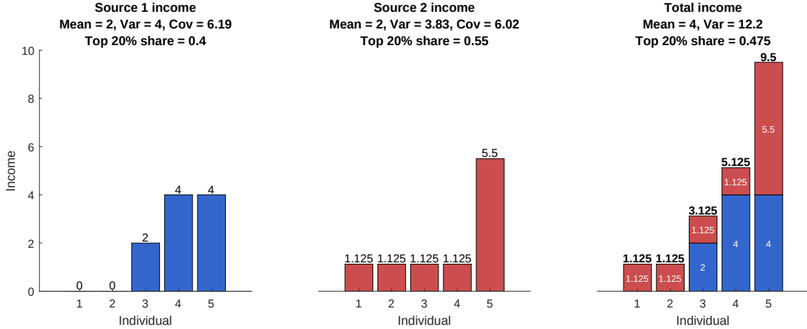
Figure 2: Income distributions of Example 2.
